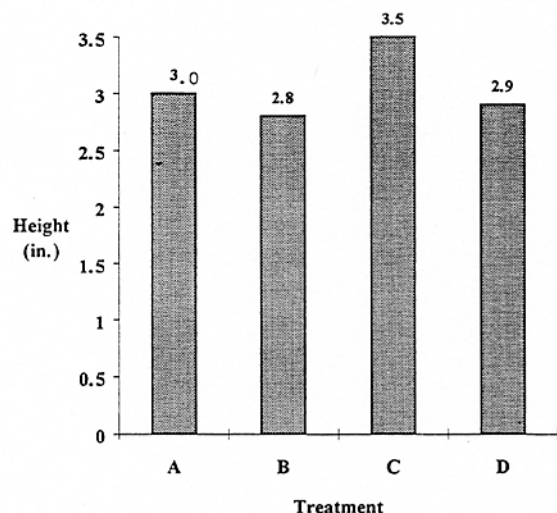
Figure 7. Average maximum height of red maple seedlings on 4 different seedbeds at 75 days after seeding for 3 ROW plant species combined (poverty grass, rough goldenrod, hayscented fern). Treatment A, undisturbed; B, exposed ROW soil; C, litter on topsoil; D, commercial topsoil.
